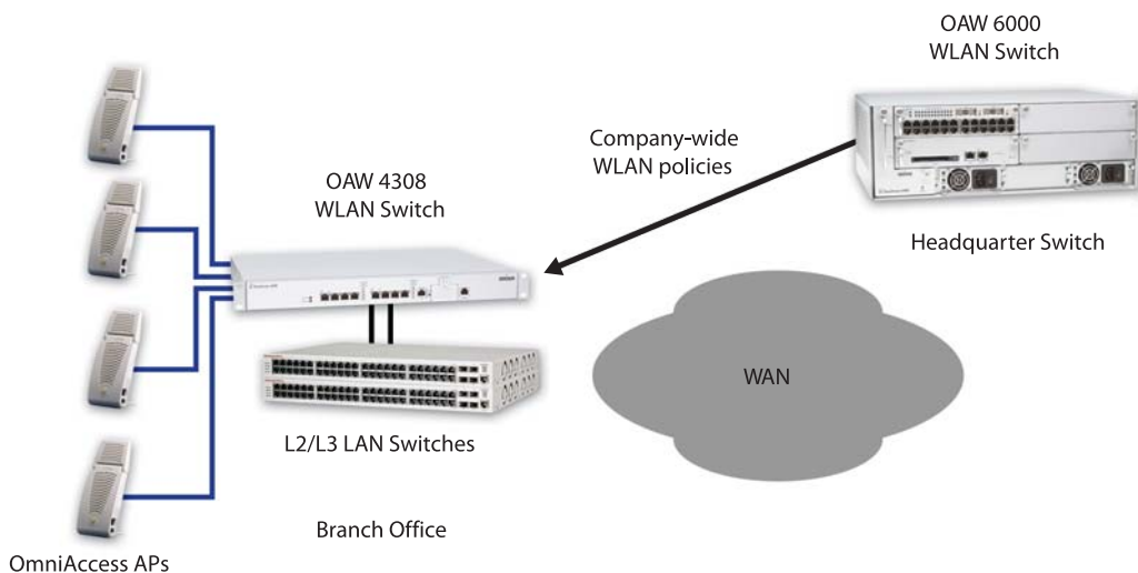
Alcatel-Lucent OmniAccess 4308 deployed as a WLAN appliance in a branch office
