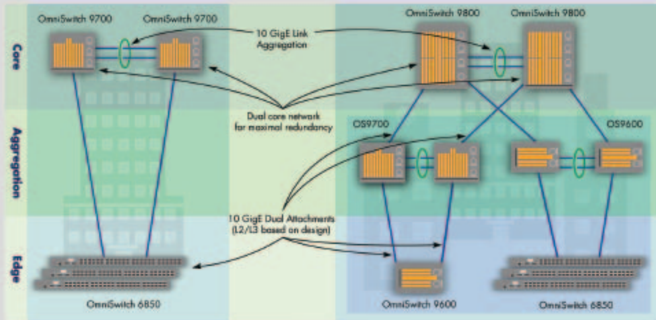
Medium-sized network Two tier, single data center/building
