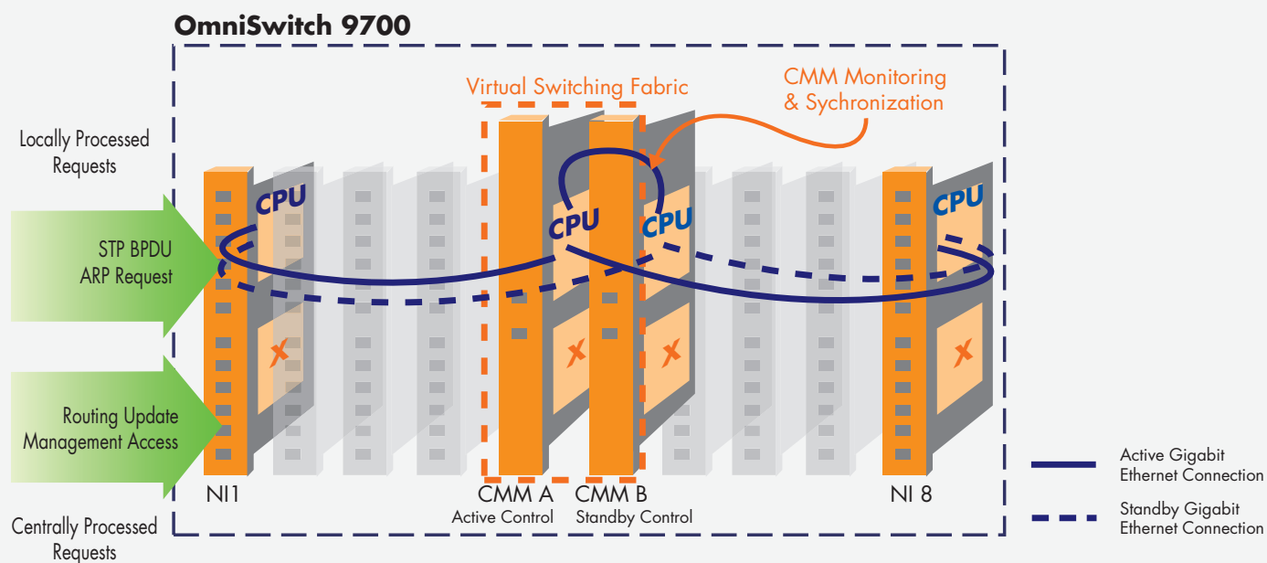
Principle of operation for distributed intelligence
